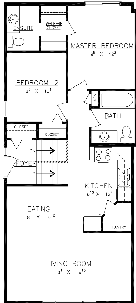
FLOOR PLAN
